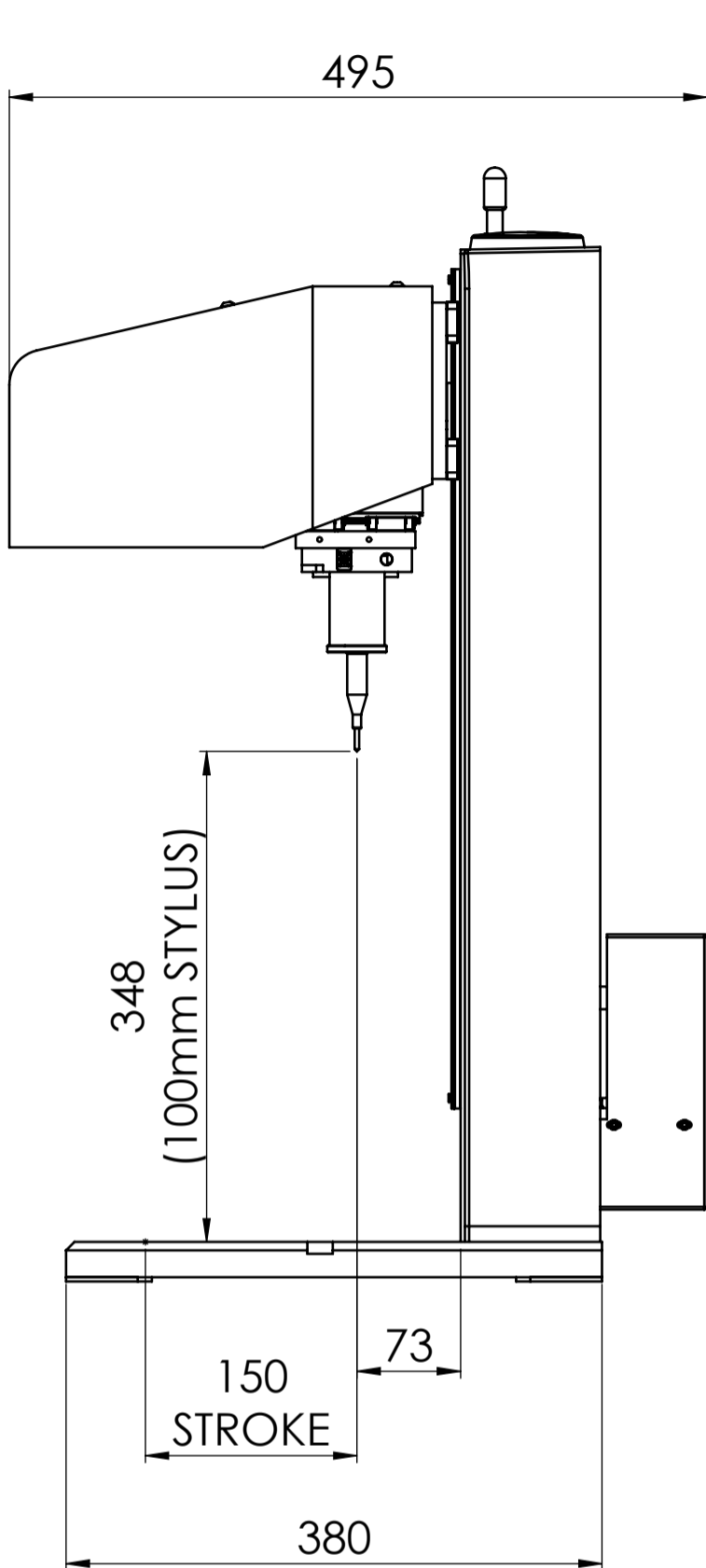
SIDE VIEW
